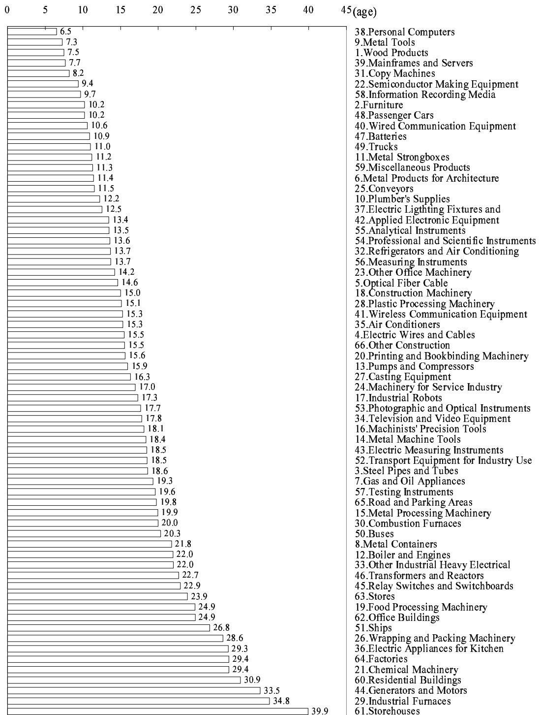
Fig. 4 Average Service Lives in Japan based on the Estimated Weibull Distribution
